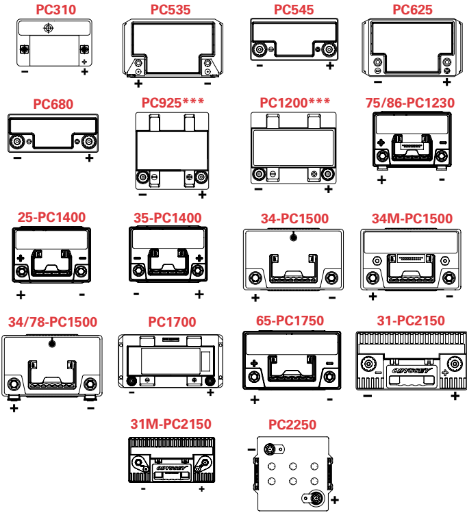
Drawing sizes are for terminal position reference only; diagrams are not proportionate to each other. ***Optional Reversed Polarity (L)
